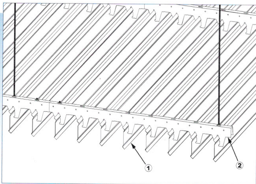
Suspension Drawing : Screening Ceiling System 吊掛示意圖：垂直片型掛式天花系統
