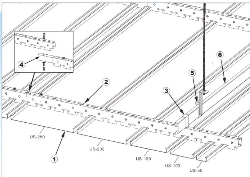
Suspension Drawing : Recessed Linear Ceiling System 吊掛示意圖：間縫條型天花系統
