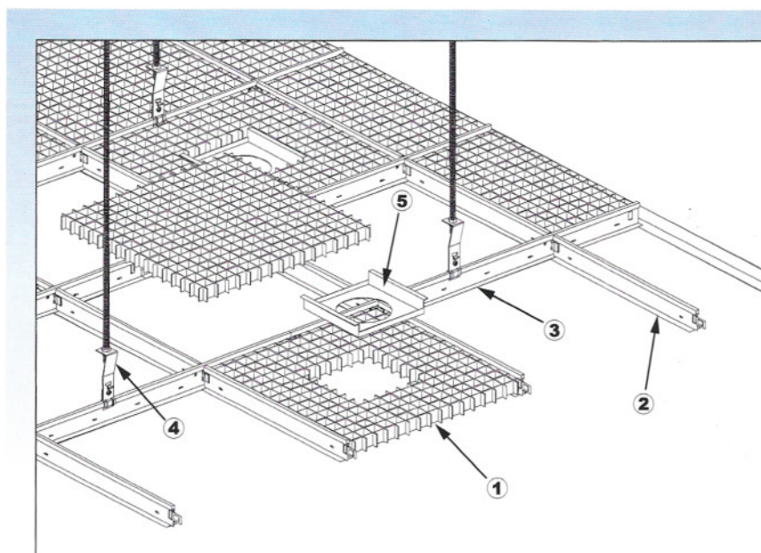
Suspension Drawing : 4000 Open Grid Ceiling System 吊掛示意圖：4000 燈片網格天花系統
