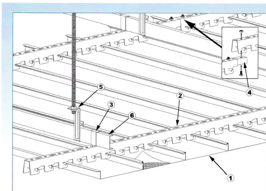
Suspension Drawing : Linear Ceiling System 吊掛示意圖：條型天花系統
